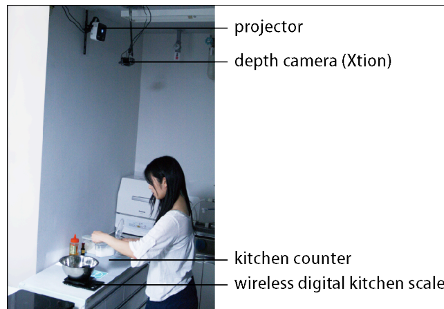
Fig. 2. Configuration of the system. The wireless digital kitchen scale tracks the quantity of an ingredient that the user has poured into the scale.
